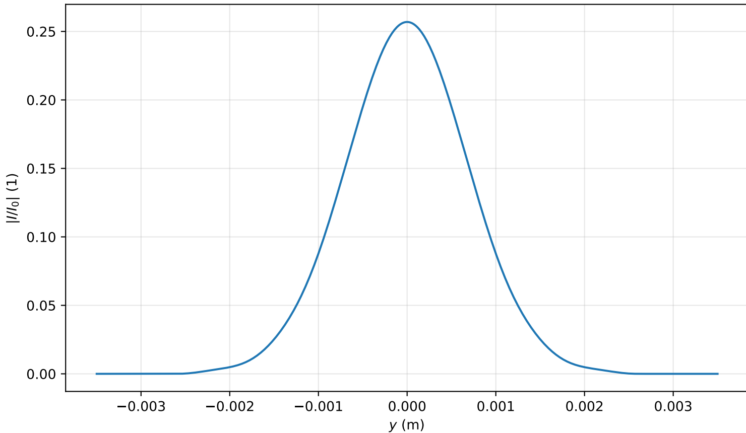
Intensity profile I(x=0, y, z=3.901)/I_0 , P_{in}=0.2P_{cr} , artificial time
